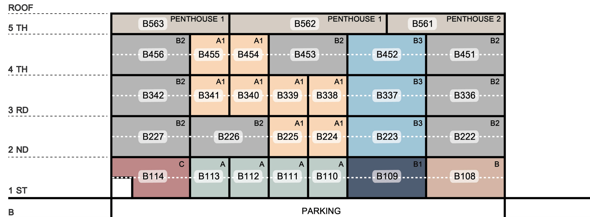
SECTION 02
